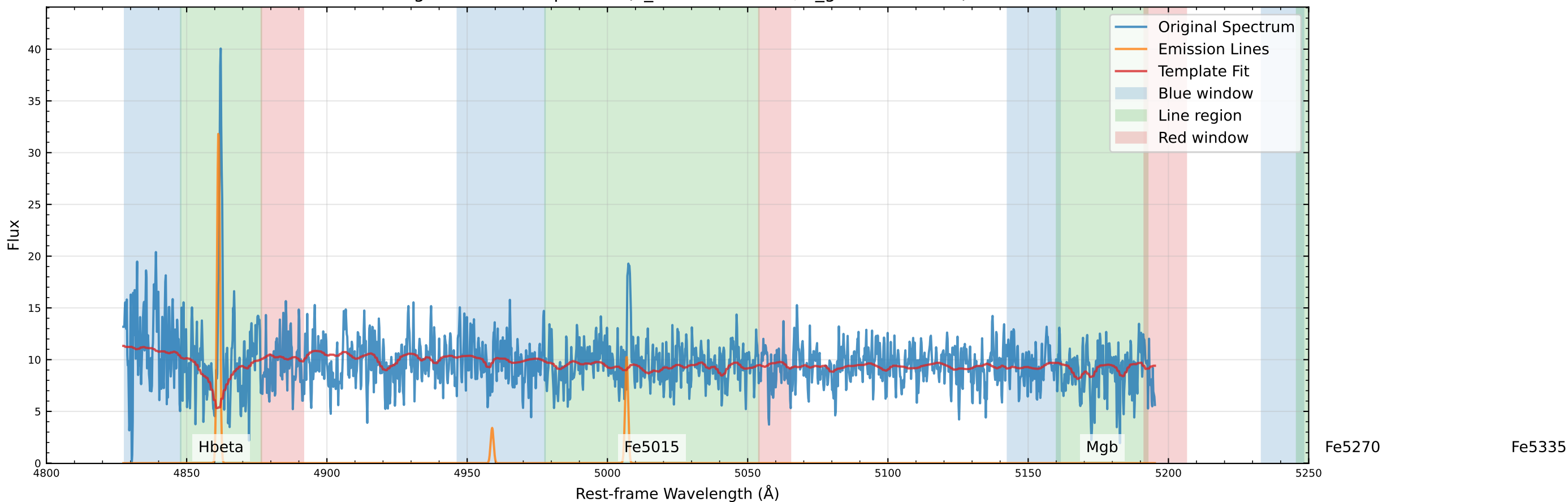
Original Data Comparison (v_star=56.5 km/s, v_gas=47.5 km/s)
