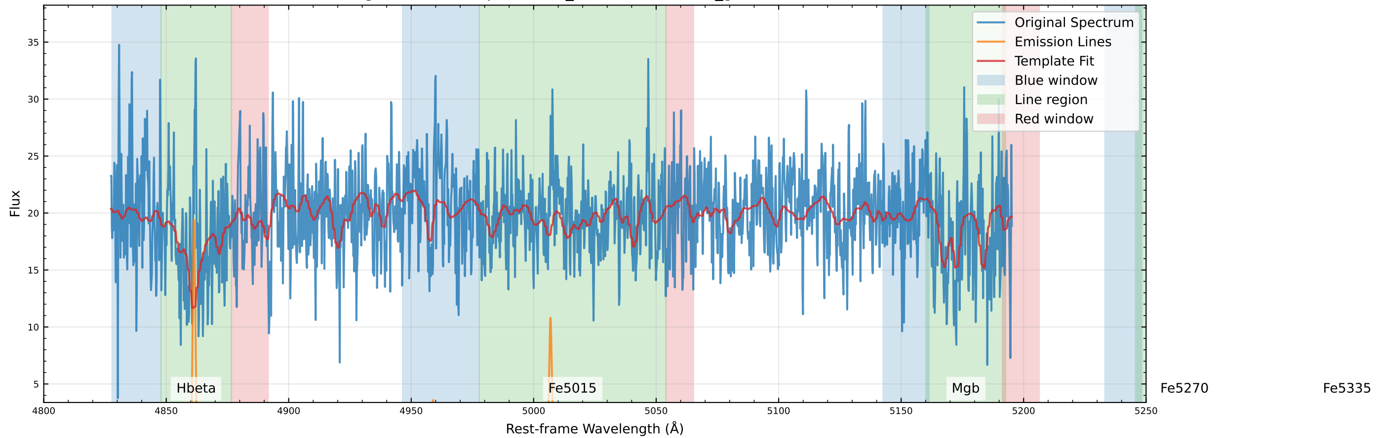
Original Data Comparison (v_star=24.2 km/s, v_gas=32.1 km/s)
