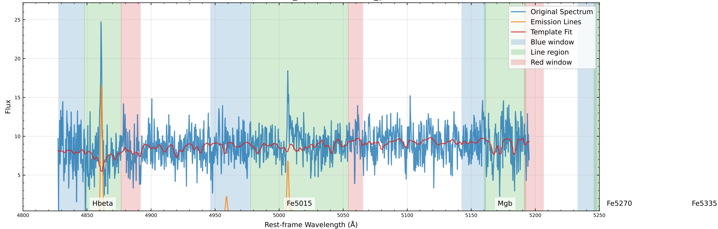
Original Data Comparison (v_star=-25.2 km/s, v_gas=-20.0 km/s)
