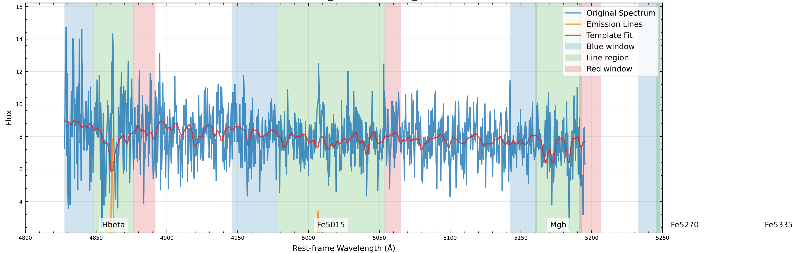
Original Data Comparison (v_star=-5.0 km/s, v_gas=16.3 km/s)
