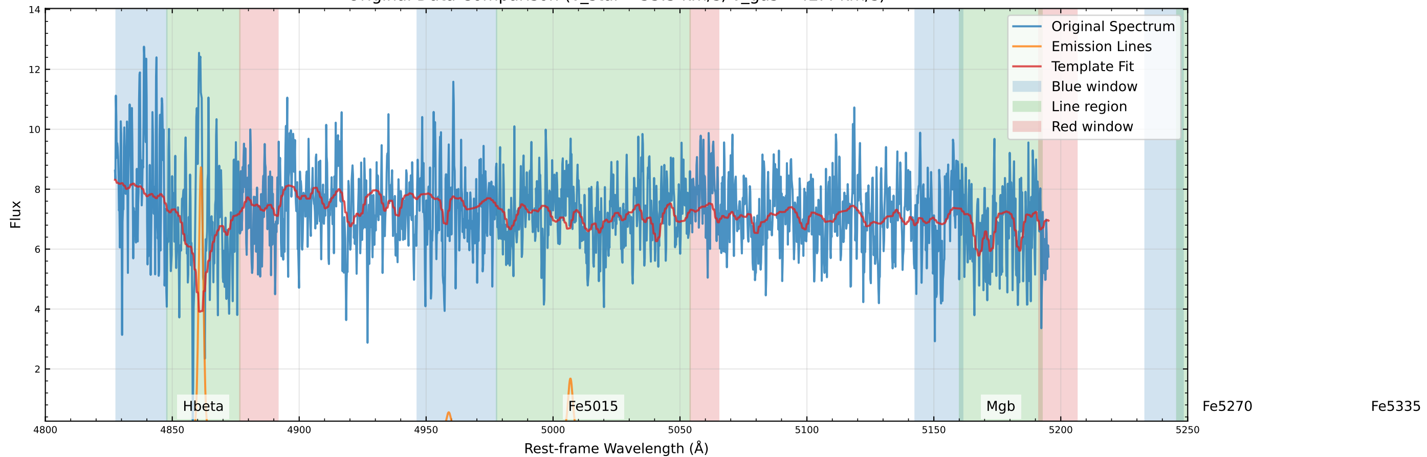
Original Data Comparison (v_star=-33.3 km/s, v_gas=-42.4 km/s)
