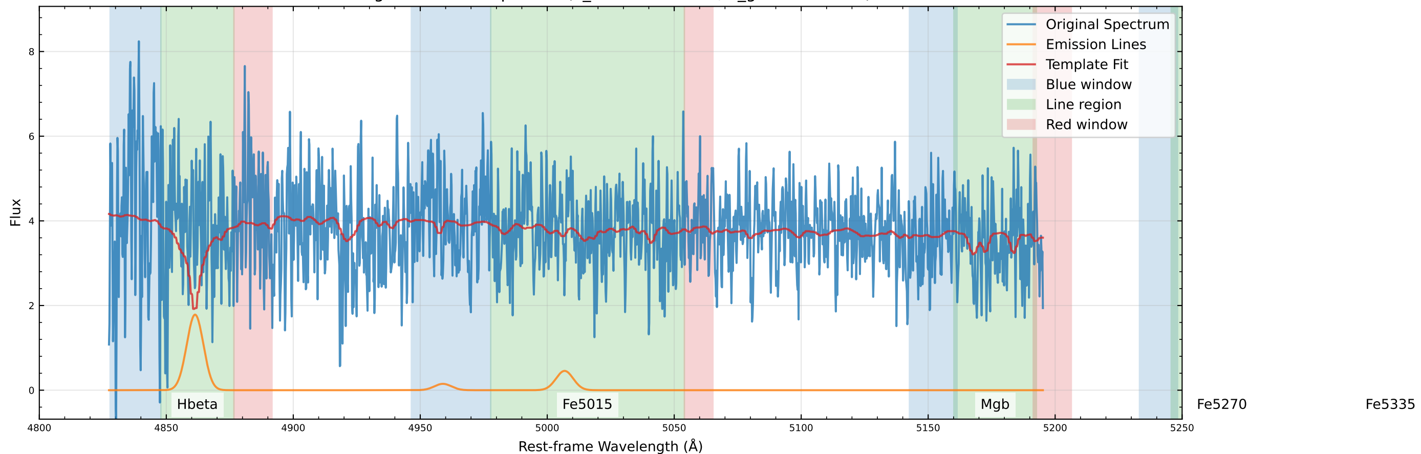
Original Data Comparison (v_star=13.9 km/s, v_gas=-5.7 km/s)
