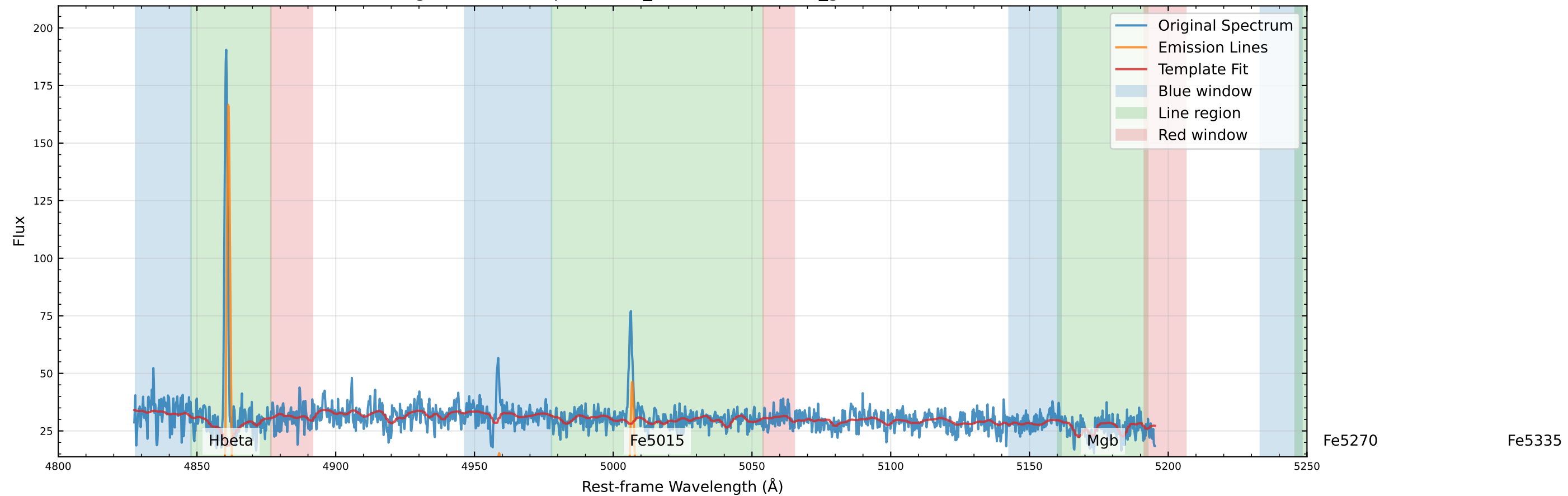
Original Data Comparison (v_star=-39.8 km/s, v_gas=-50.5 km/s)
