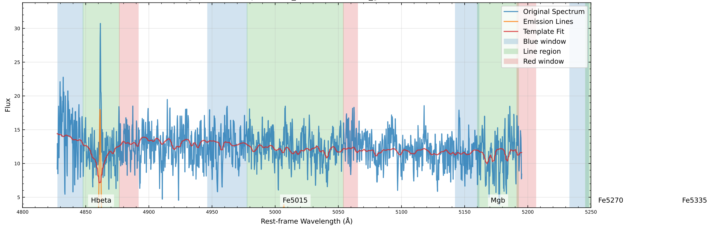
Original Data Comparison (v_star=23.4 km/s, v_gas=25.8 km/s)
