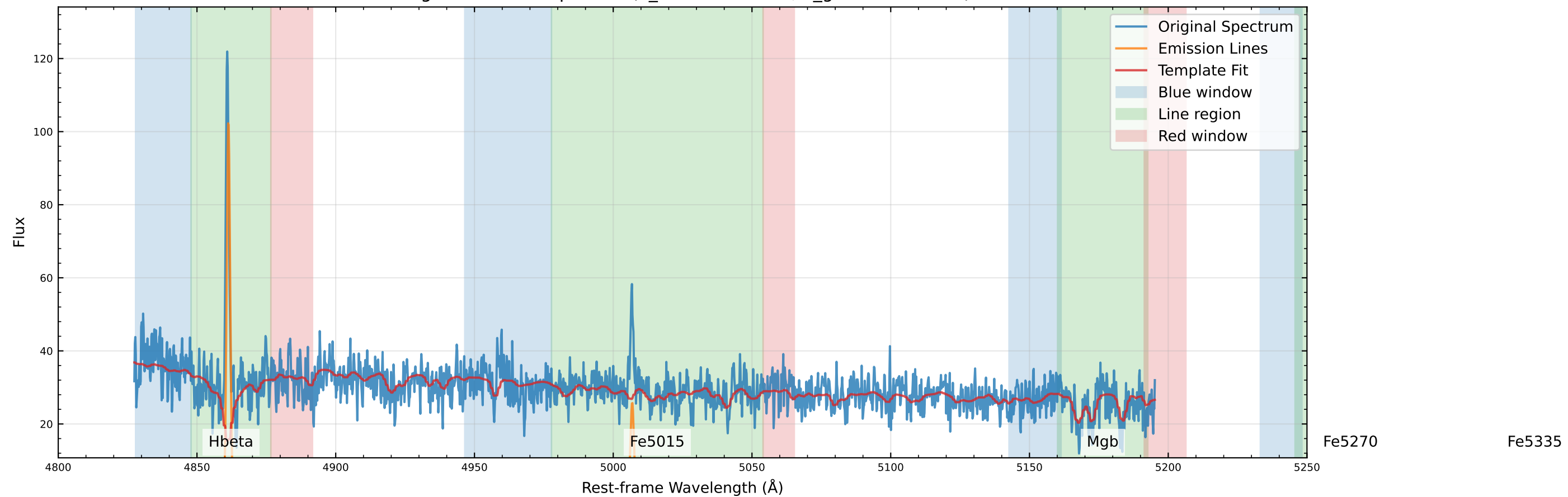
Original Data Comparison (v_star=-0.3 km/s, v_gas=-22.2 km/s)
