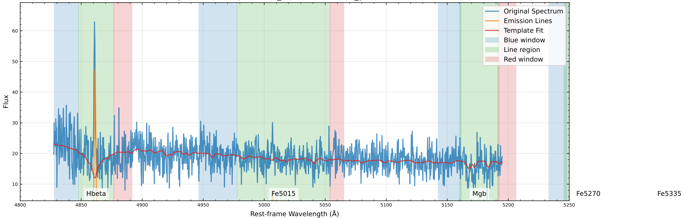
Original Data Comparison (v_star=-23.8 km/s, v_gas=-25.7 km/s)
