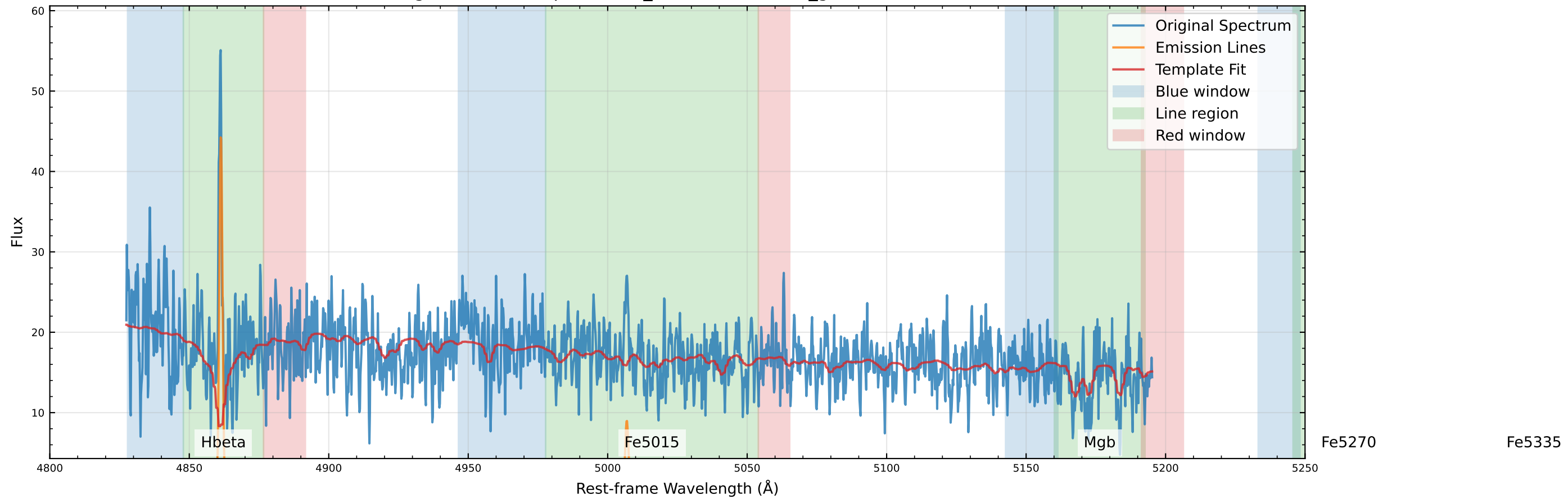
Original Data Comparison (v_star=-5.3 km/s, v_gas=-15.4 km/s)
