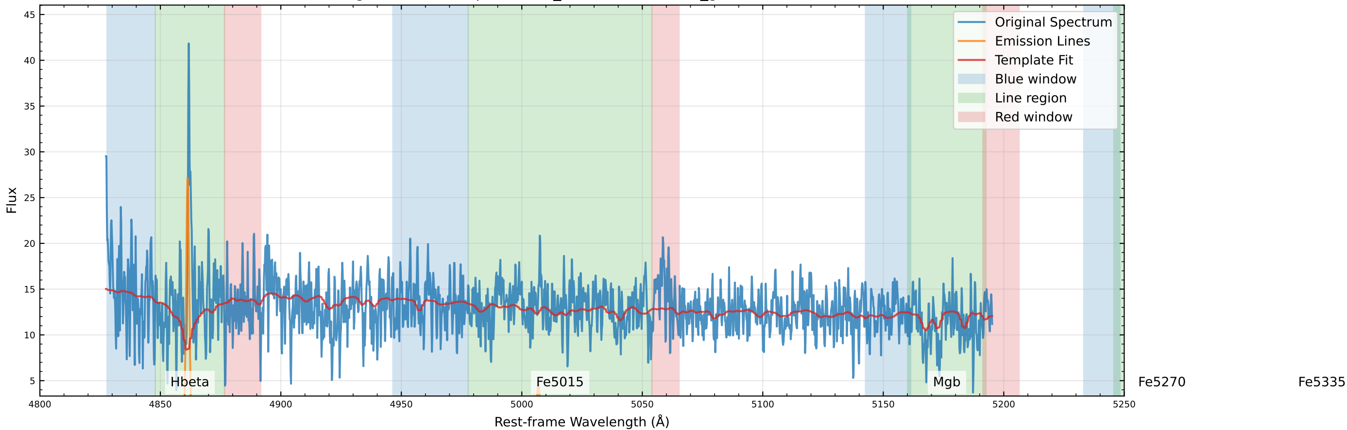
Original Data Comparison (v_star=32.7 km/s, v_gas=41.2 km/s)
