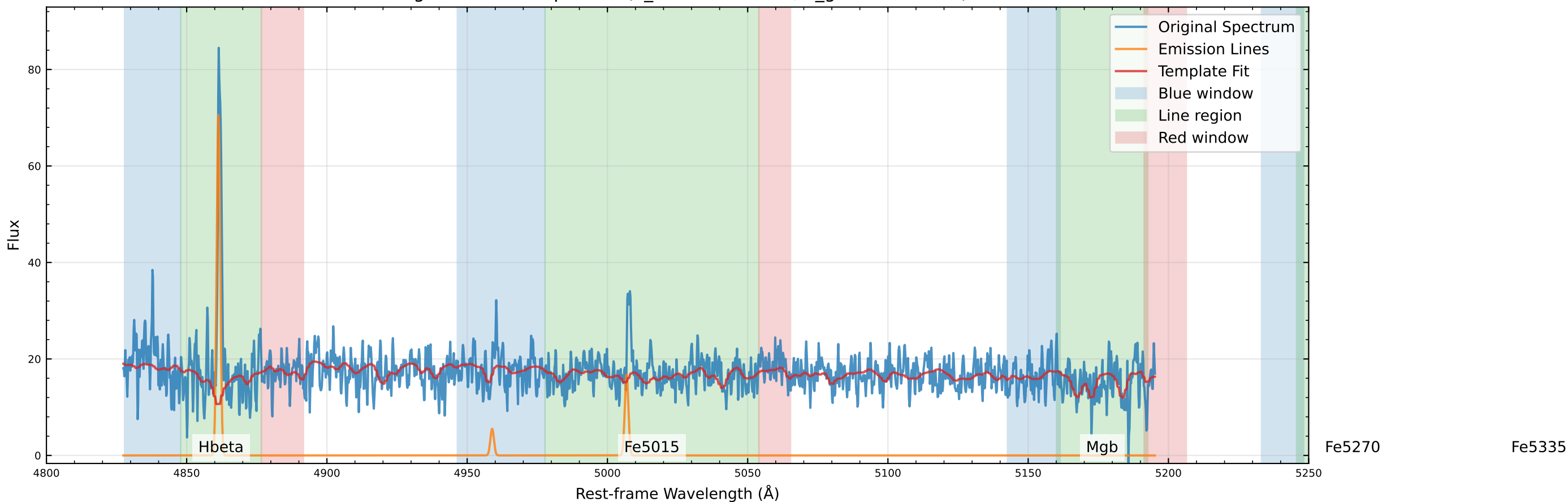
Original Data Comparison (v_star=33.3 km/s, v_gas=26.5 km/s)
