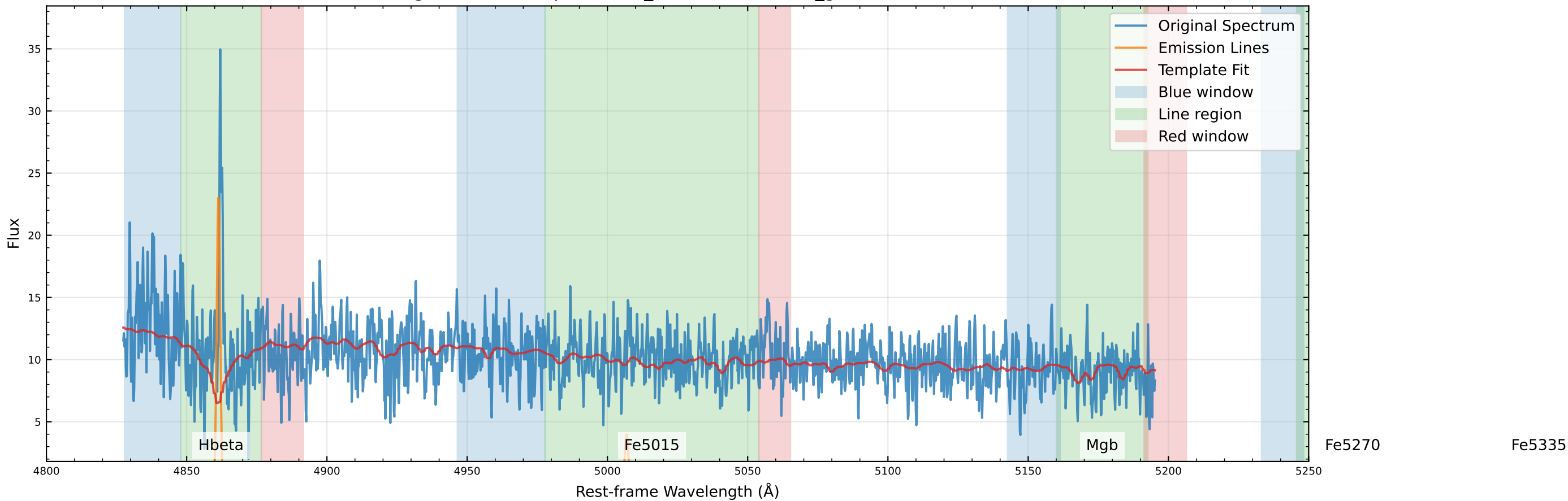
Original Data Comparison (v_star=44.3 km/s, v_gas=54.0 km/s)
