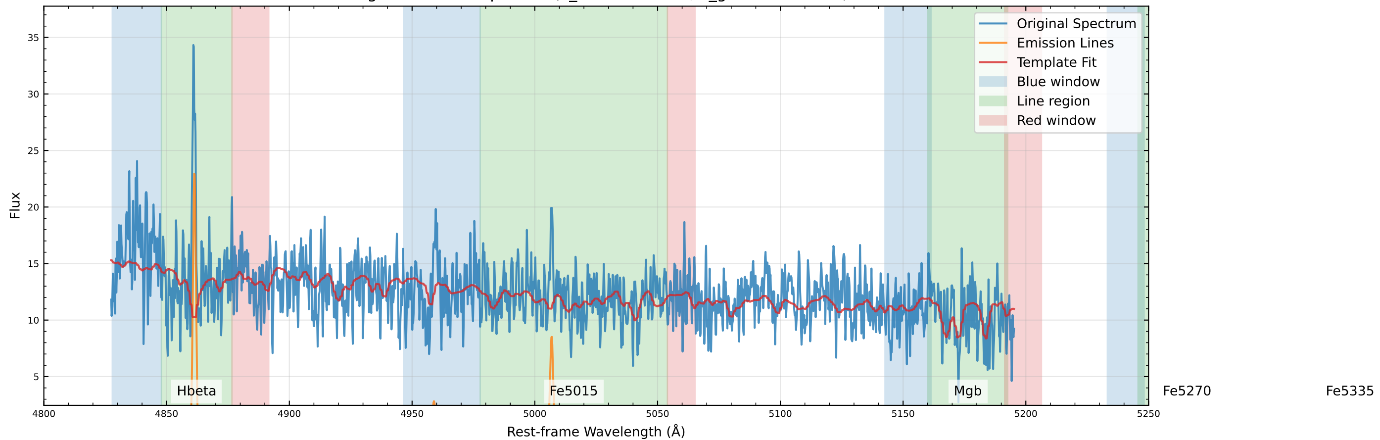
Original Data Comparison (v_star=4.7 km/s, v_gas=-10.6 km/s)
