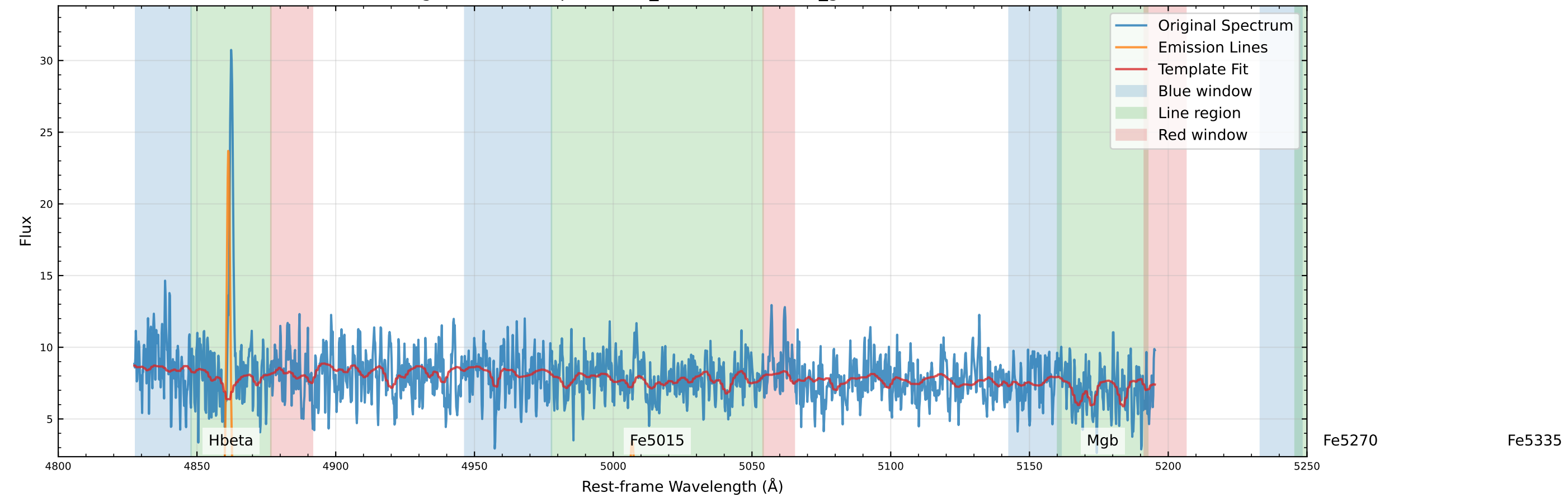
Original Data Comparison (v_star=58.8 km/s, v_gas=65.7 km/s)
