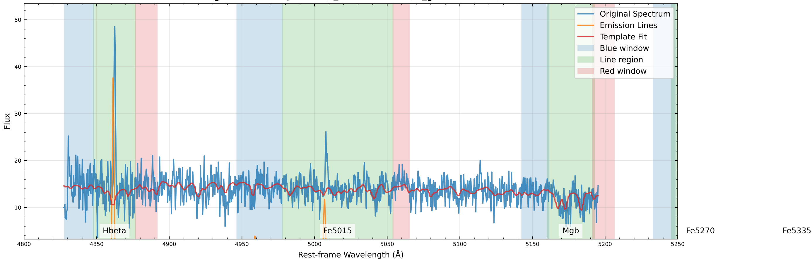
Original Data Comparison (v_star=56.1 km/s, v_gas=63.5 km/s)
