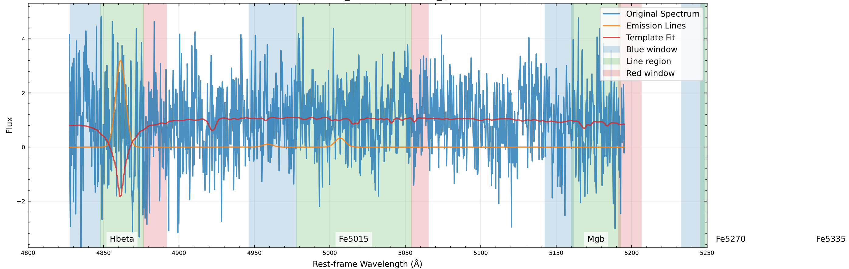
Original Data Comparison ( v_{\text{star}}=23.0 km/s, v_{\text{gas}}=-159.2 km/s)
