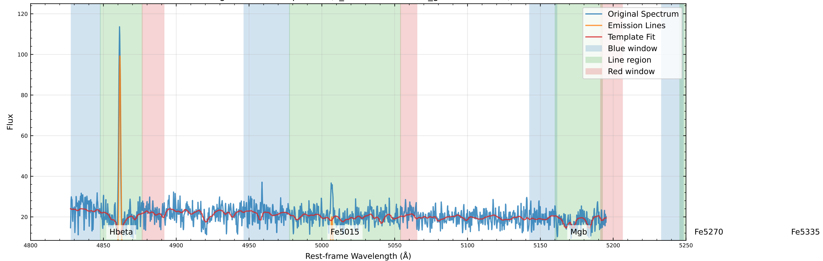
Original Data Comparison (v_star=10.5 km/s, v_gas=-14.3 km/s)
