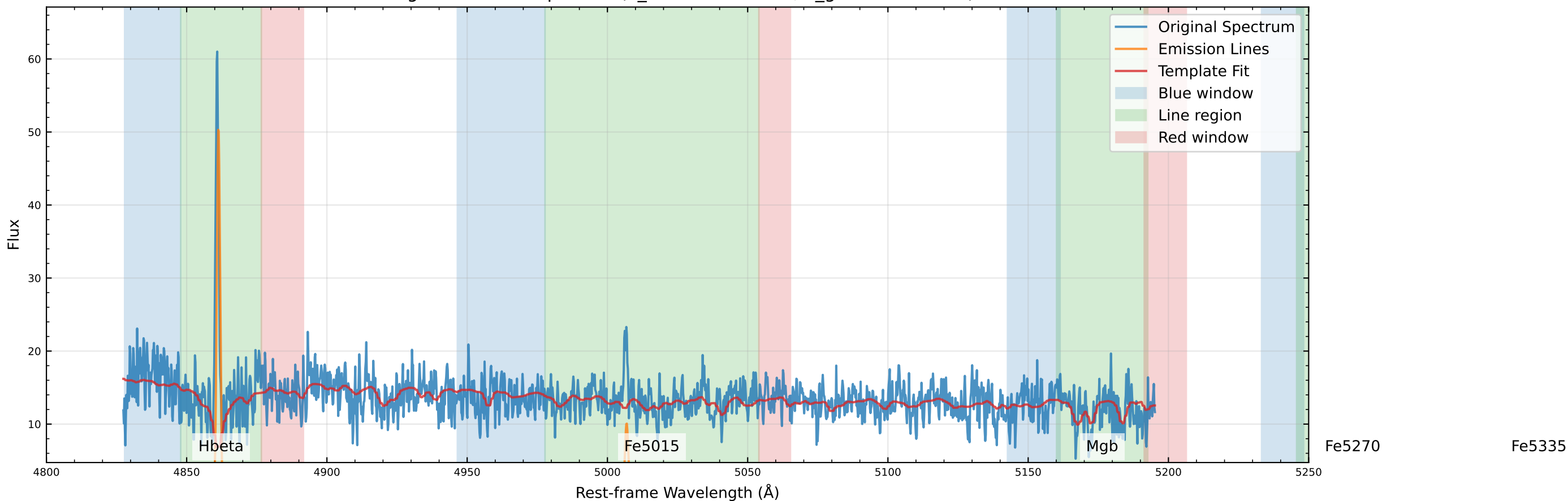
Original Data Comparison (v_star=-19.1 km/s, v_gas=-29.0 km/s)
