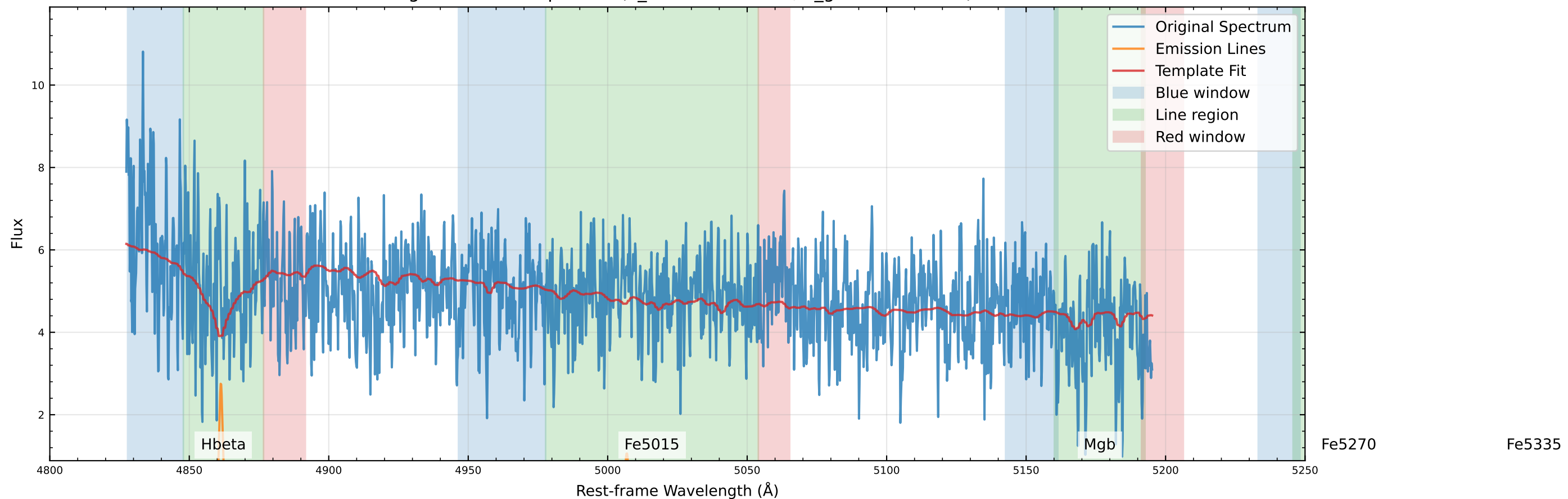
Original Data Comparison (v_star=-84.4 km/s, v_gas=-46.0 km/s)
