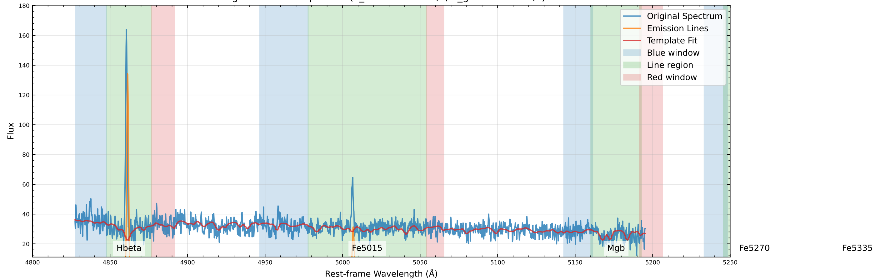
Original Data Comparison (v_star=-24.5 km/s, v_gas=-46.6 km/s)
