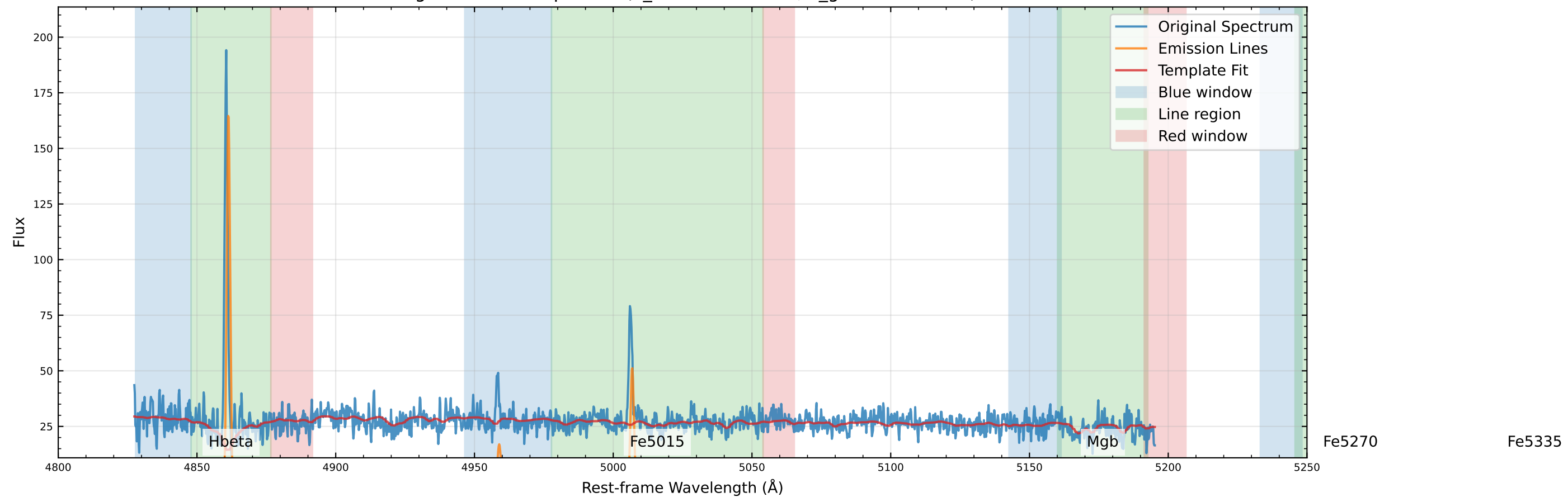
Original Data Comparison (v_star=-42.9 km/s, v_gas=-49.7 km/s)
