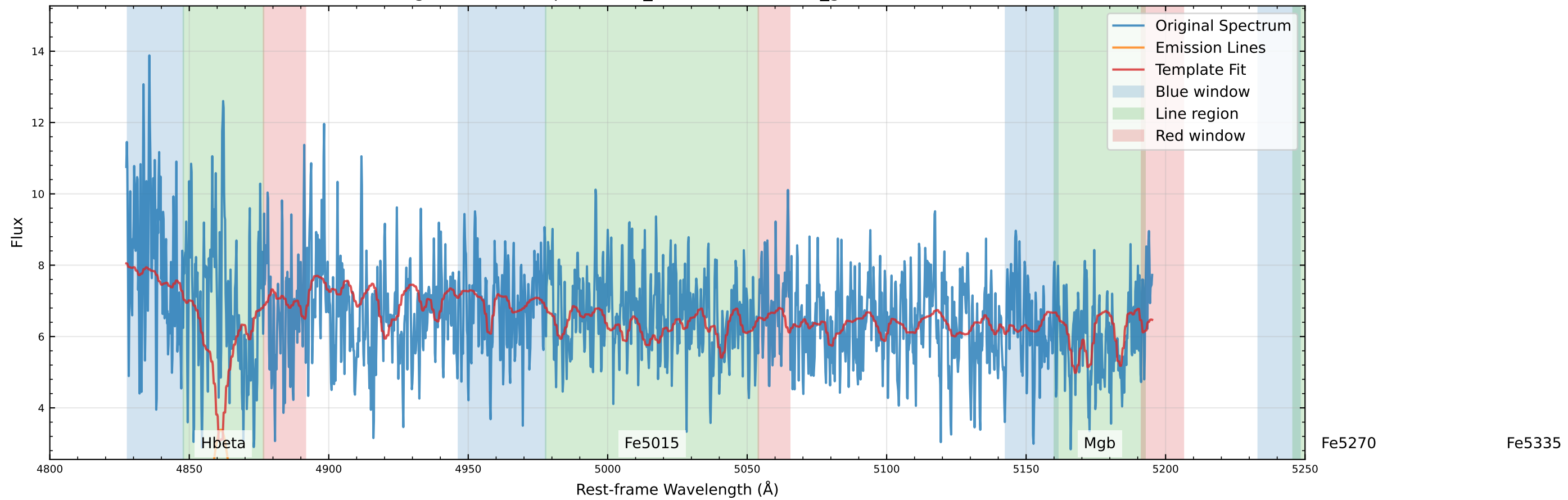
Original Data Comparison (v_star=-74.1 km/s, v_gas=-3.9 km/s)
