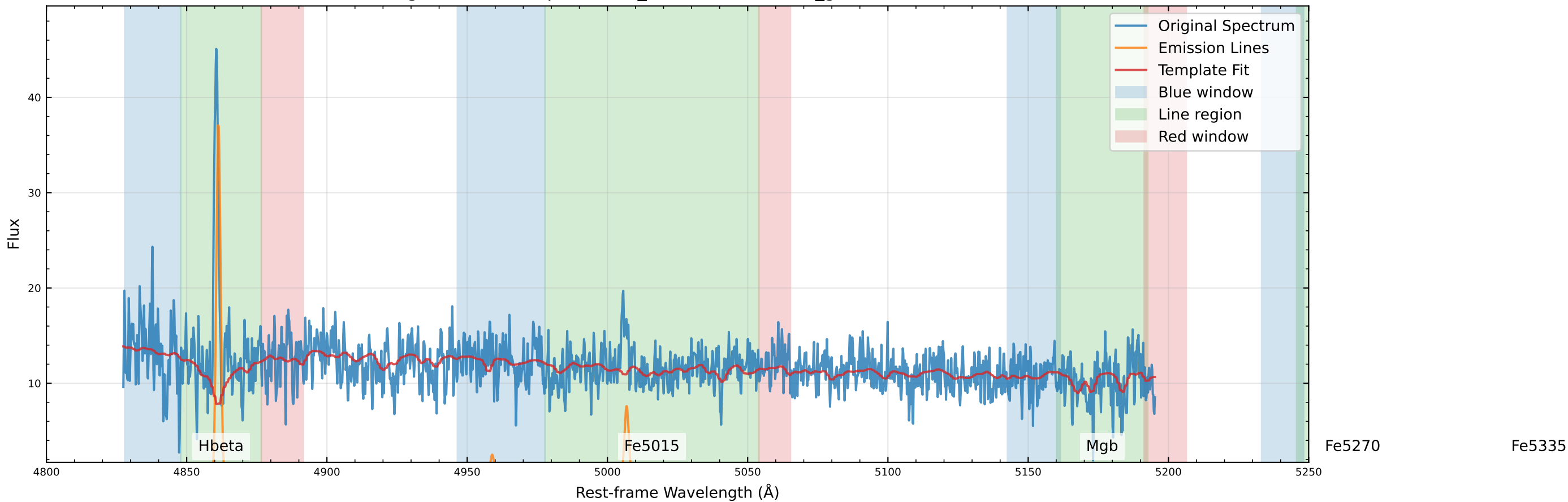
Original Data Comparison (v_star=-27.2 km/s, v_gas=-47.1 km/s)
