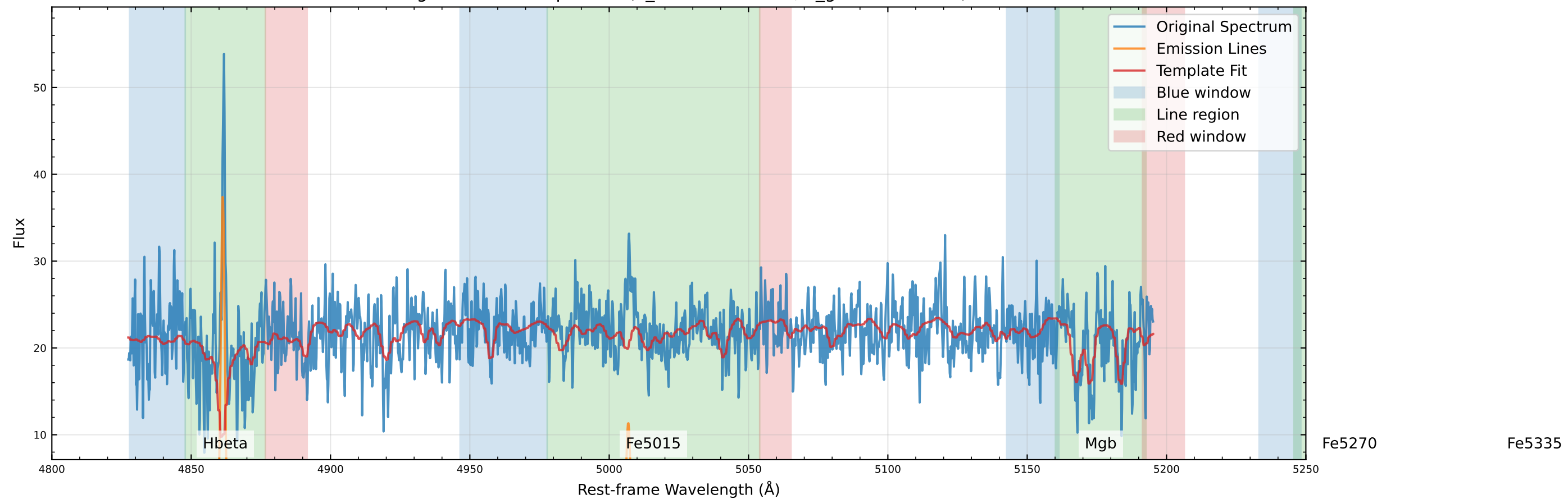
Original Data Comparison (v_star=33.2 km/s, v_gas=20.6 km/s)
