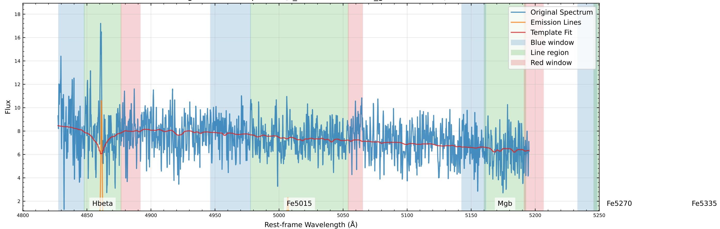
Original Data Comparison (v_star=-15.8 km/s, v_gas=-28.6 km/s)
