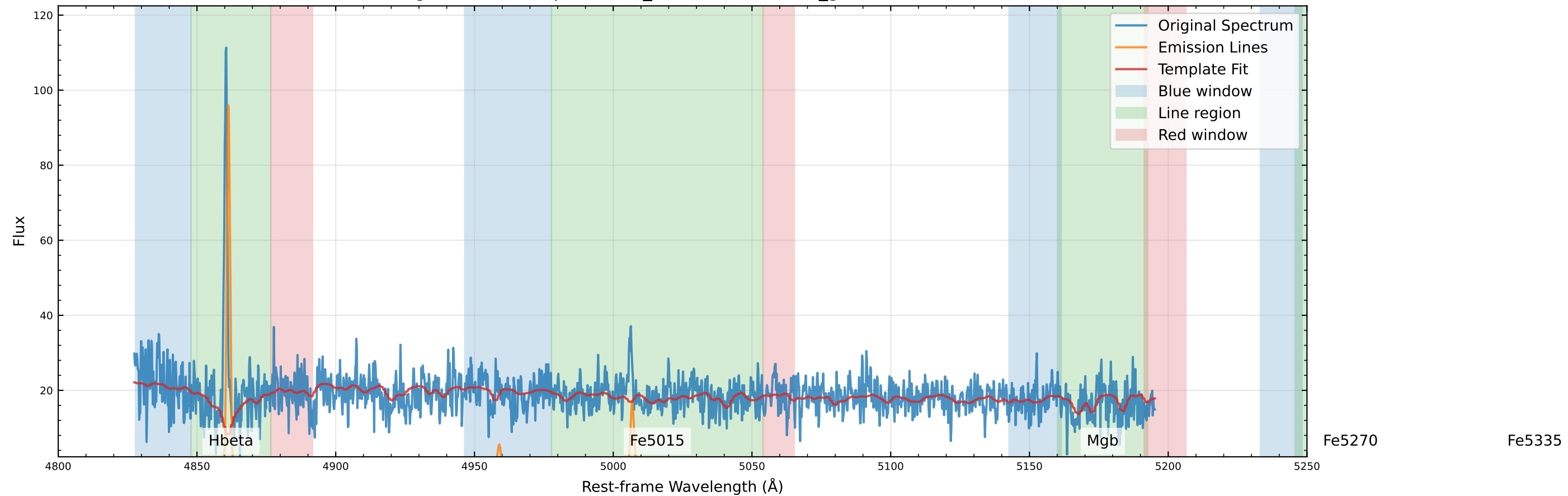
Original Data Comparison (v_star=-42.1 km/s, v_gas=-57.7 km/s)
