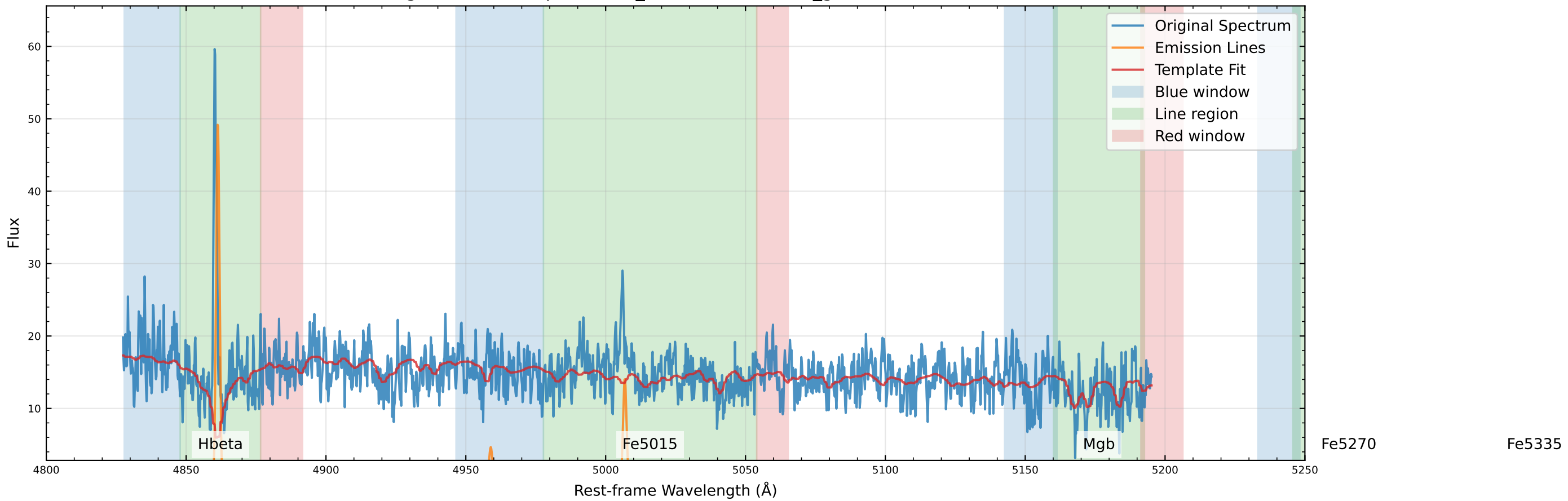
Original Data Comparison (v_star=-42.0 km/s, v_gas=-58.1 km/s)
