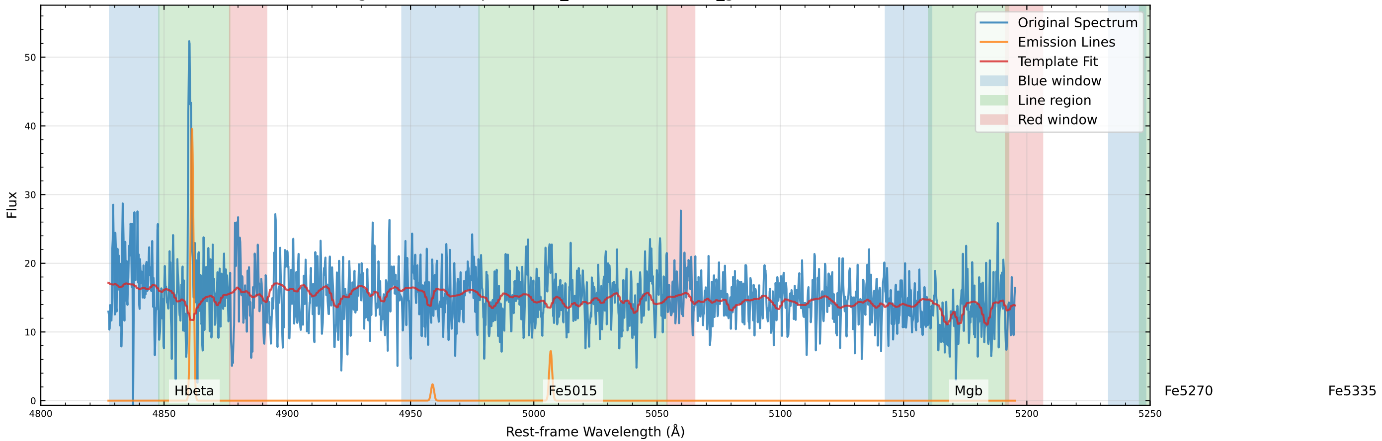
Original Data Comparison (v_star=-29.6 km/s, v_gas=-53.6 km/s)
