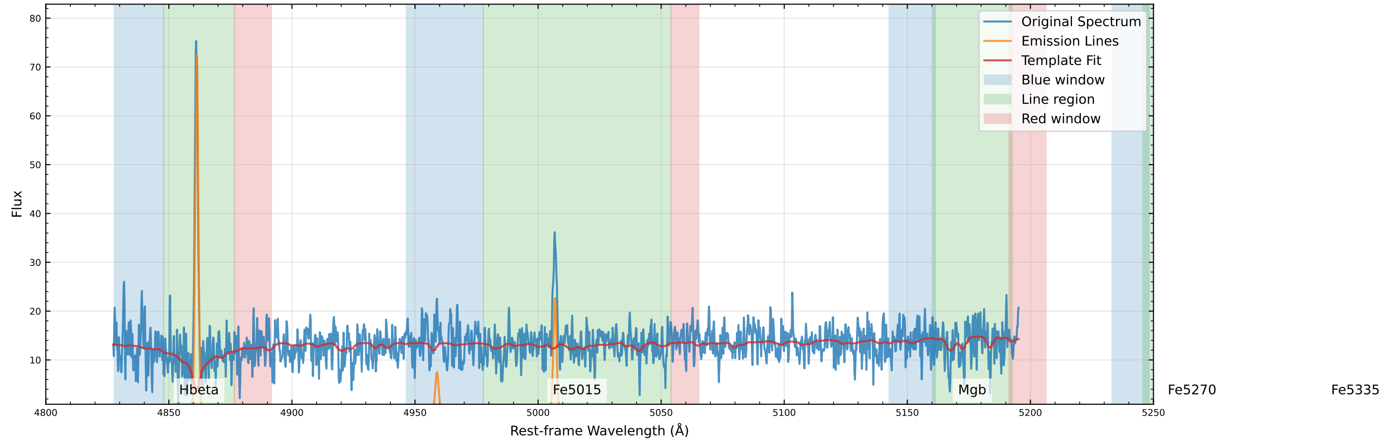
Original Data Comparison (v_star=-5.3 km/s, v_gas=-11.0 km/s)
