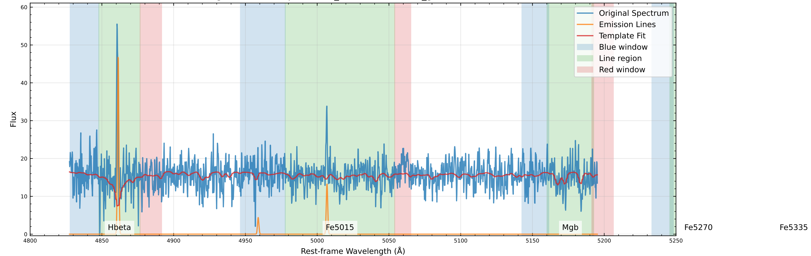
Original Data Comparison (v_star=12.2 km/s, v_gas=-37.3 km/s)
