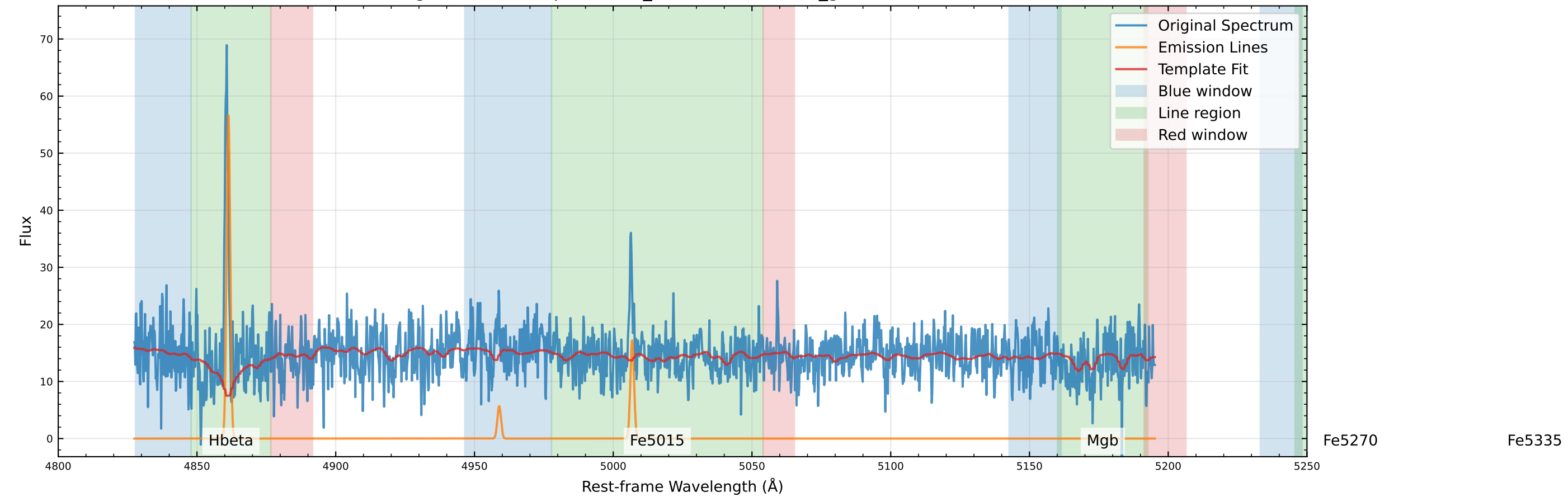
Original Data Comparison (v_star=-45.7 km/s, v_gas=-40.1 km/s)
