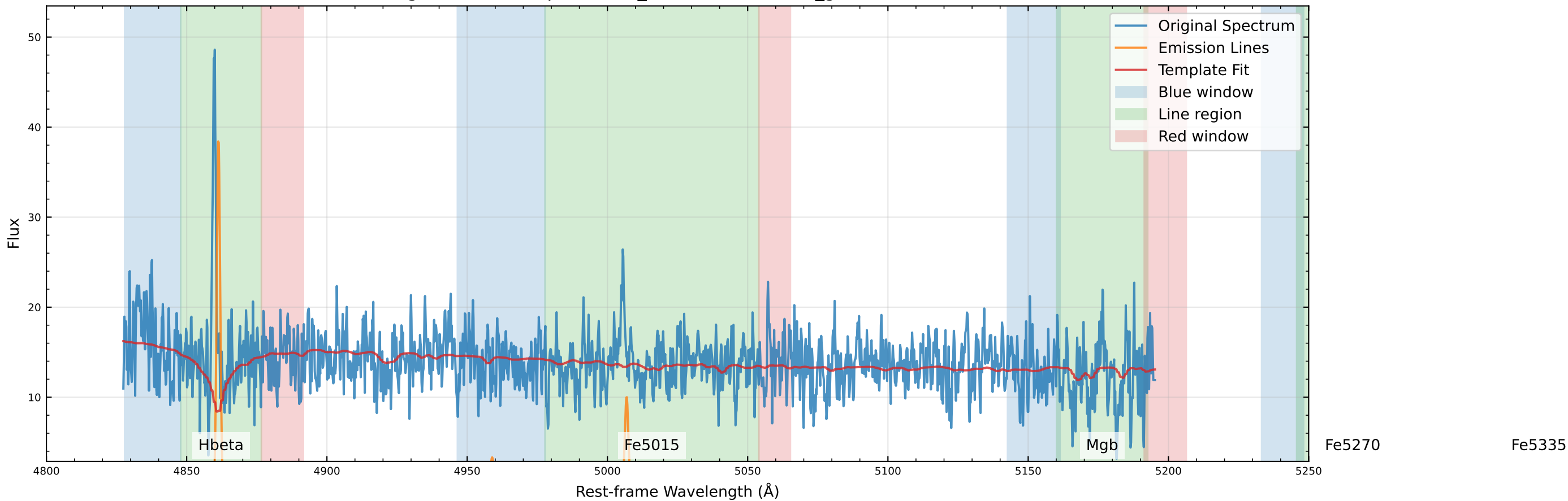
Original Data Comparison (v_star=-84.4 km/s, v_gas=-93.0 km/s)
