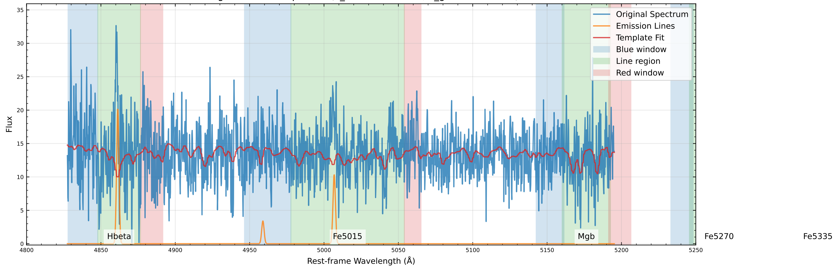
Original Data Comparison (v_star=-45.4 km/s, v_gas=-53.5 km/s)
