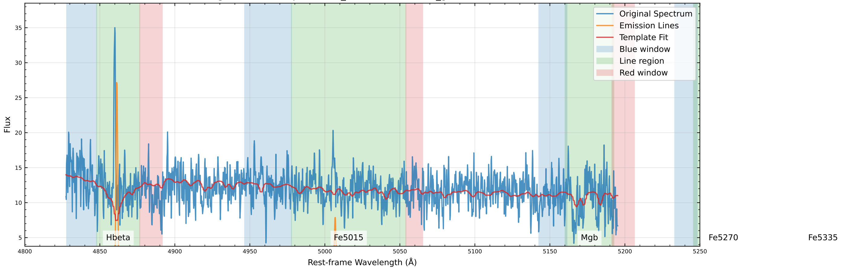
Original Data Comparison (v_star=-77.7 km/s, v_gas=-88.4 km/s)
