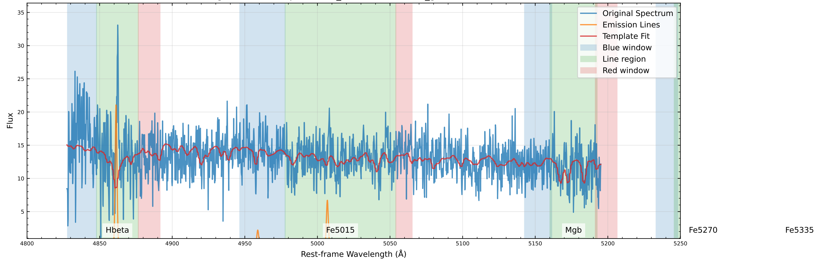
Original Data Comparison (v_star=54.1 km/s, v_gas=64.0 km/s)
