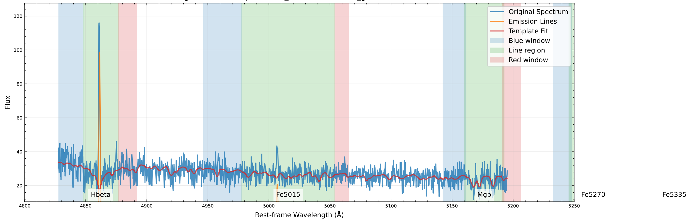
Original Data Comparison (v_star=-4.3 km/s, v_gas=-21.8 km/s)
