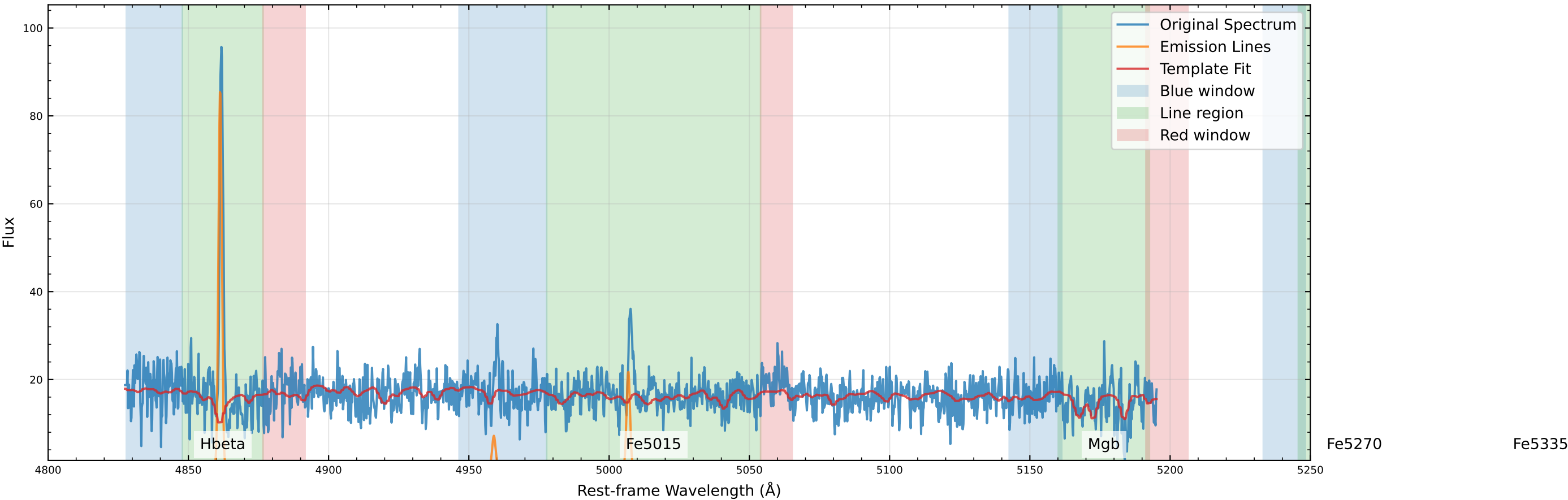
Original Data Comparison (v_star=42.3 km/s, v_gas=29.8 km/s)
