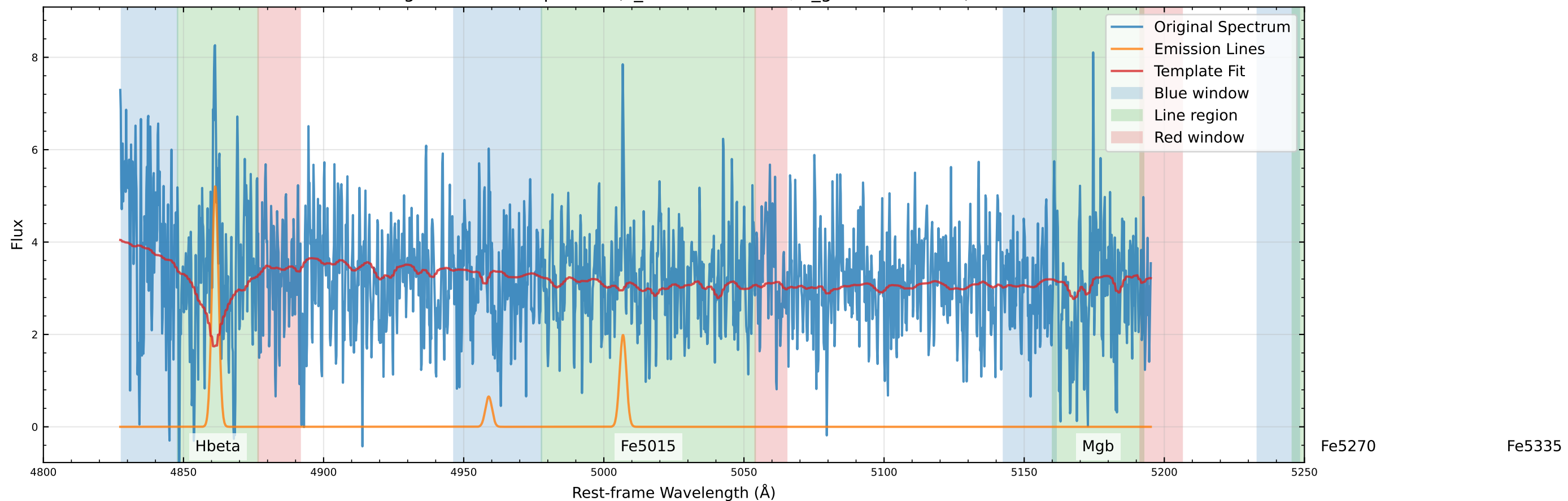
Original Data Comparison (v_star=-31.7 km/s, v_gas=-12.4 km/s)
