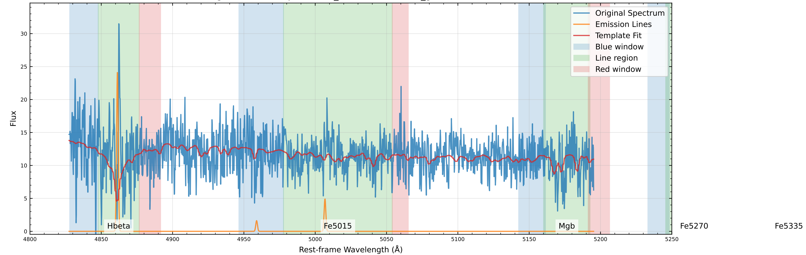
Original Data Comparison (v_star=88.0 km/s, v_gas=78.3 km/s)
