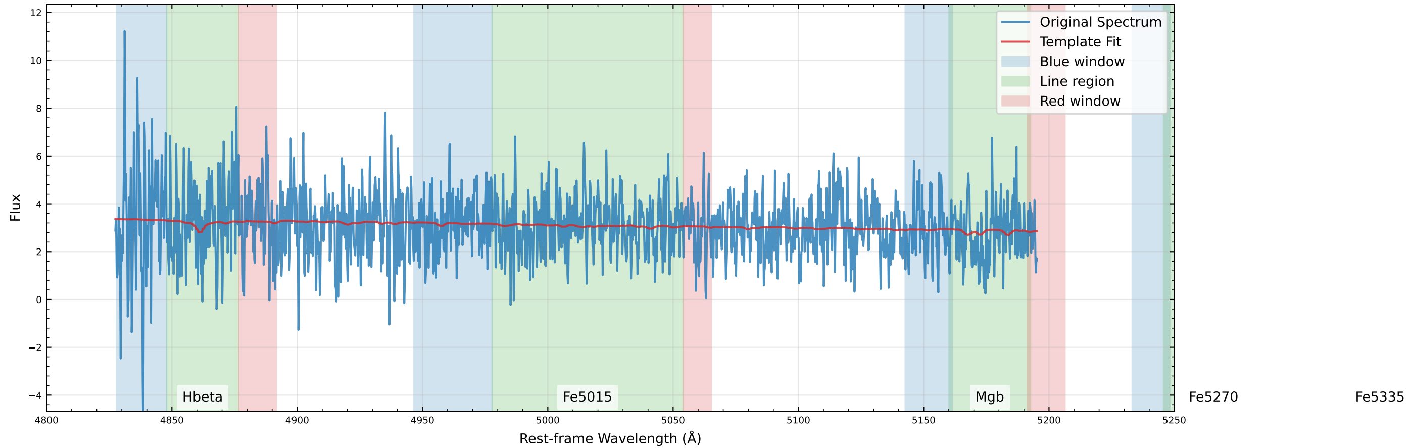
Original Data Comparison (v_star=96.7 km/s, v_gas=95.1 km/s)
