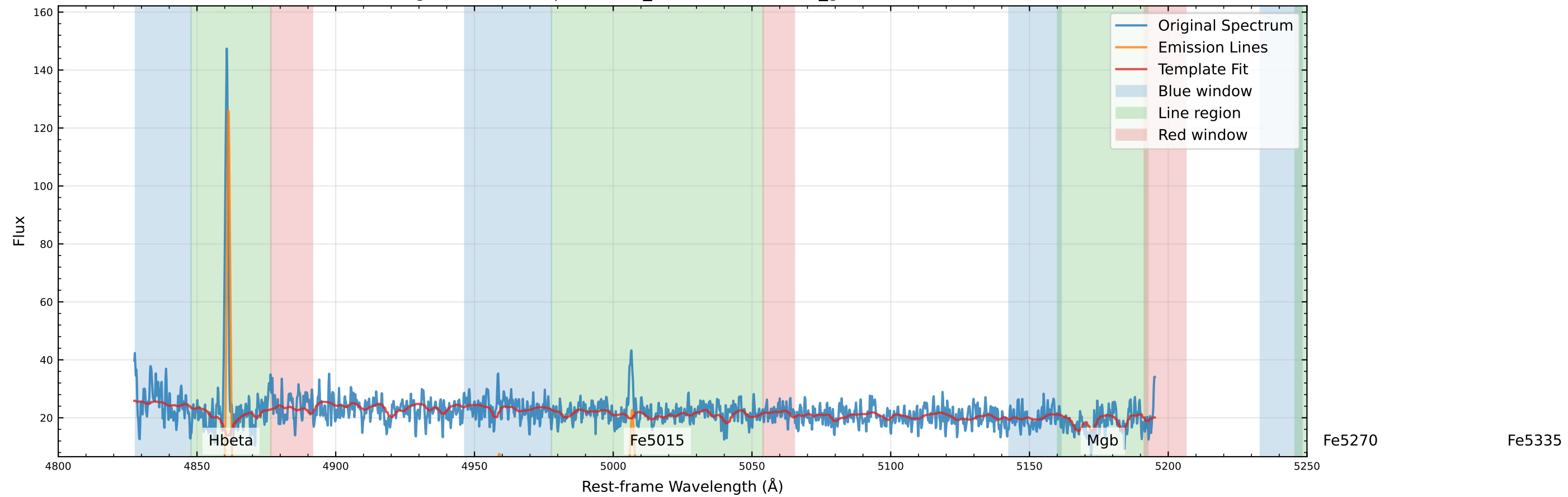
Original Data Comparison (v_star=-34.7 km/s, v_gas=-39.3 km/s)
