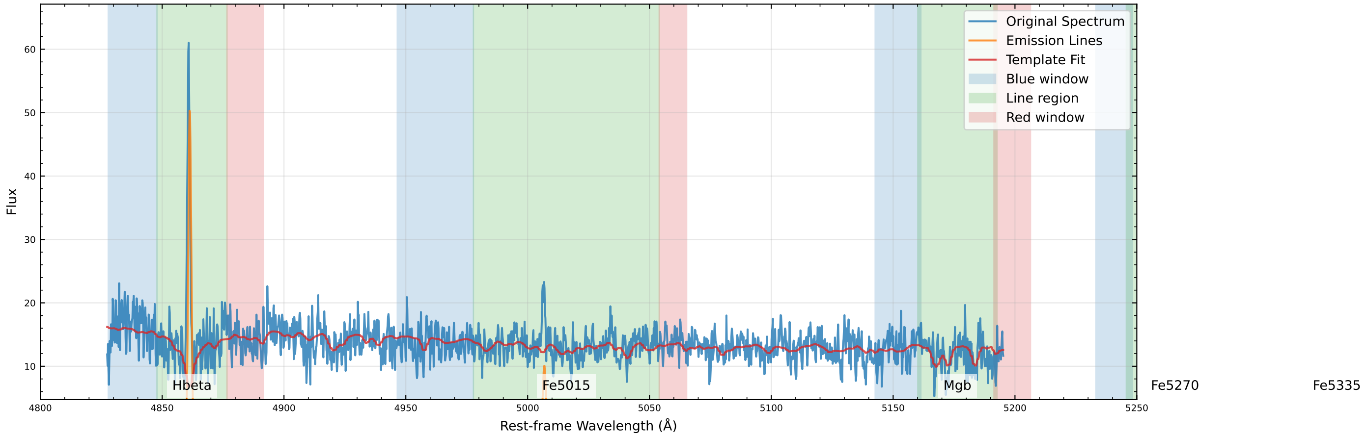
Original Data Comparison (v_star=-19.1 km/s, v_gas=-29.0 km/s)
