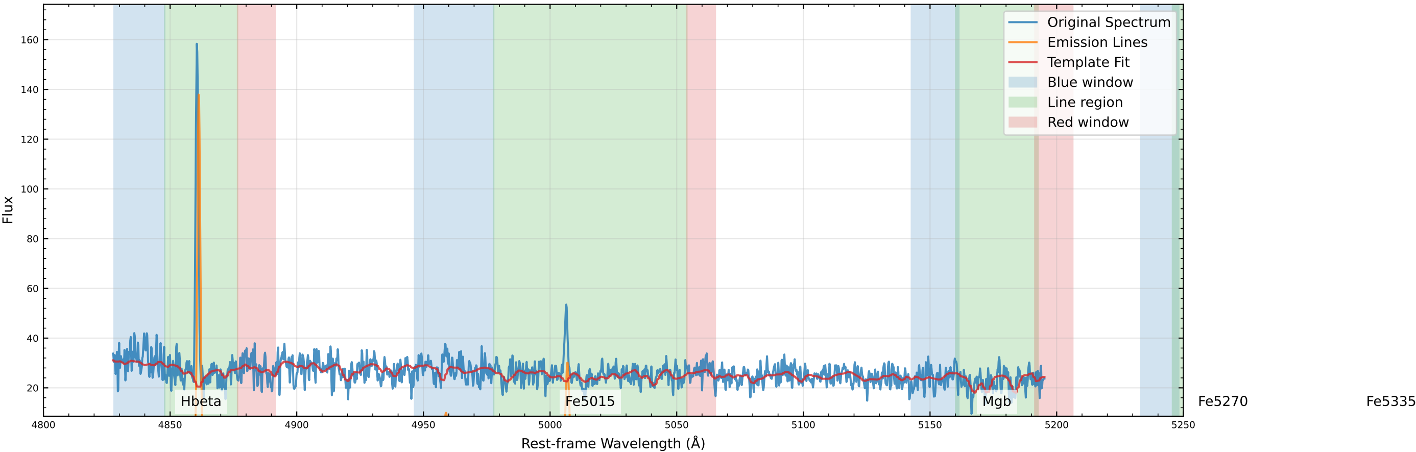
Original Data Comparison (v_star=-35.8 km/s, v_gas=-42.7 km/s)
