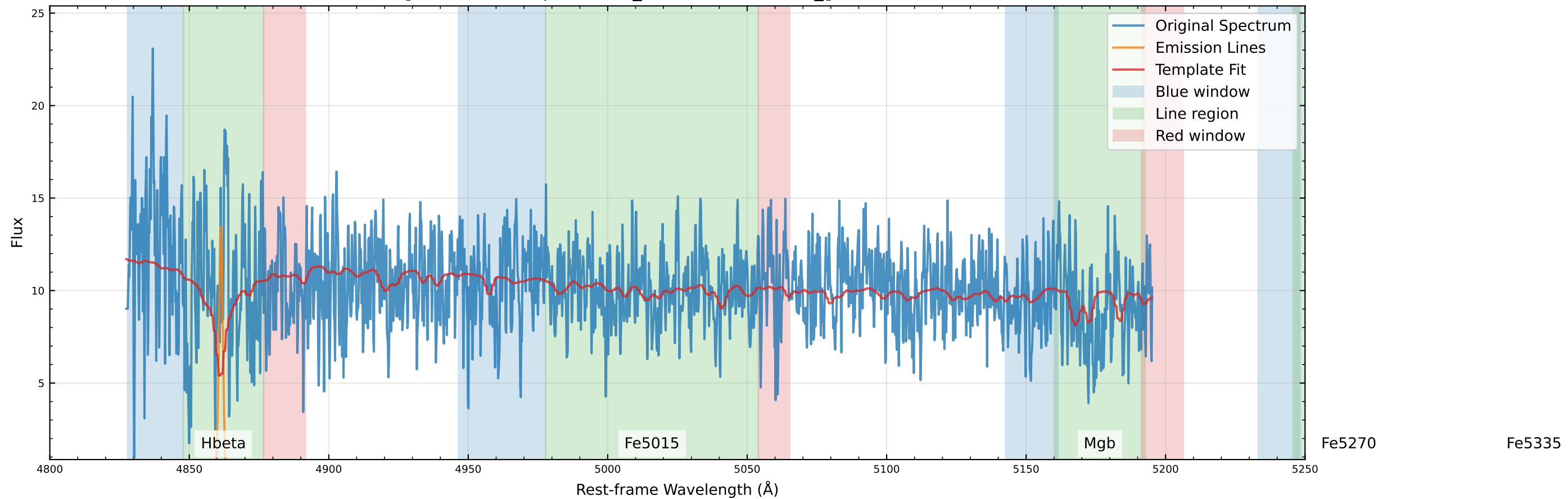
Original Data Comparison (v_star=144.6 km/s, v_gas=107.4 km/s)
