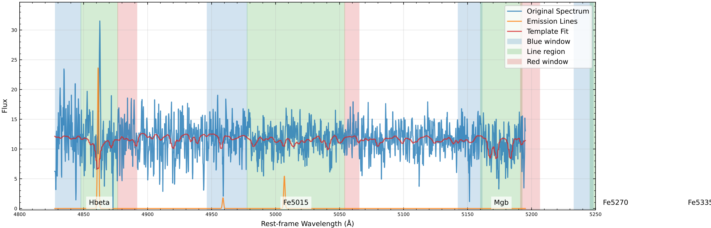
Original Data Comparison (v_star=82.5 km/s, v_gas=77.0 km/s)
