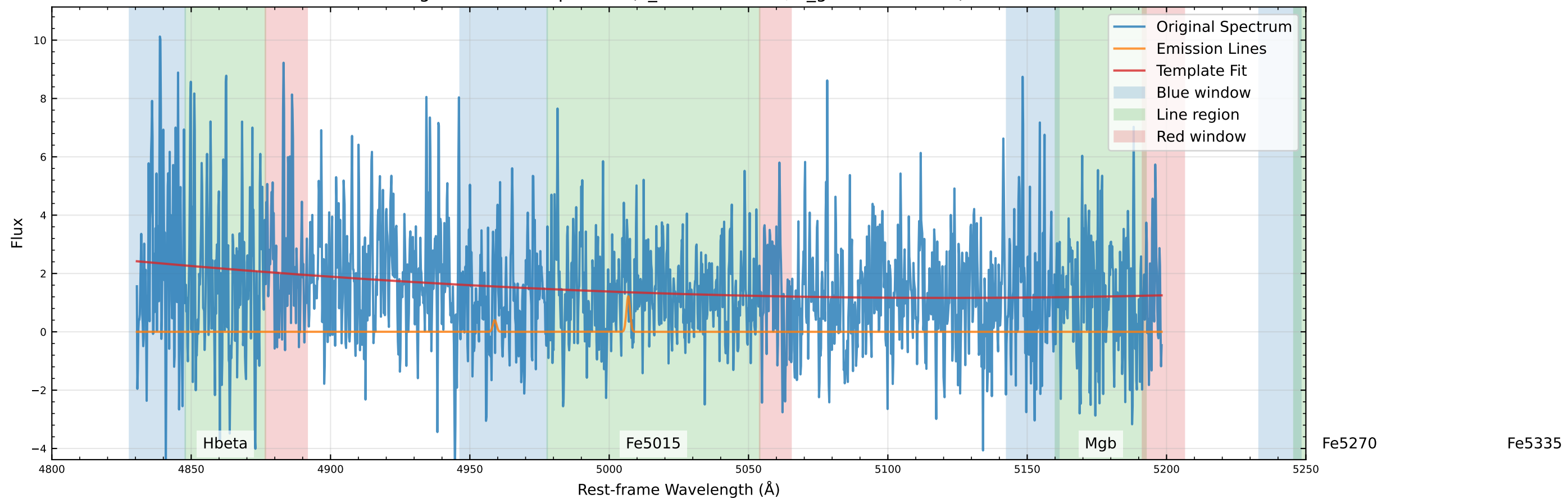
Original Data Comparison (v_star=0.0 km/s, v_gas=-31.7 km/s)
