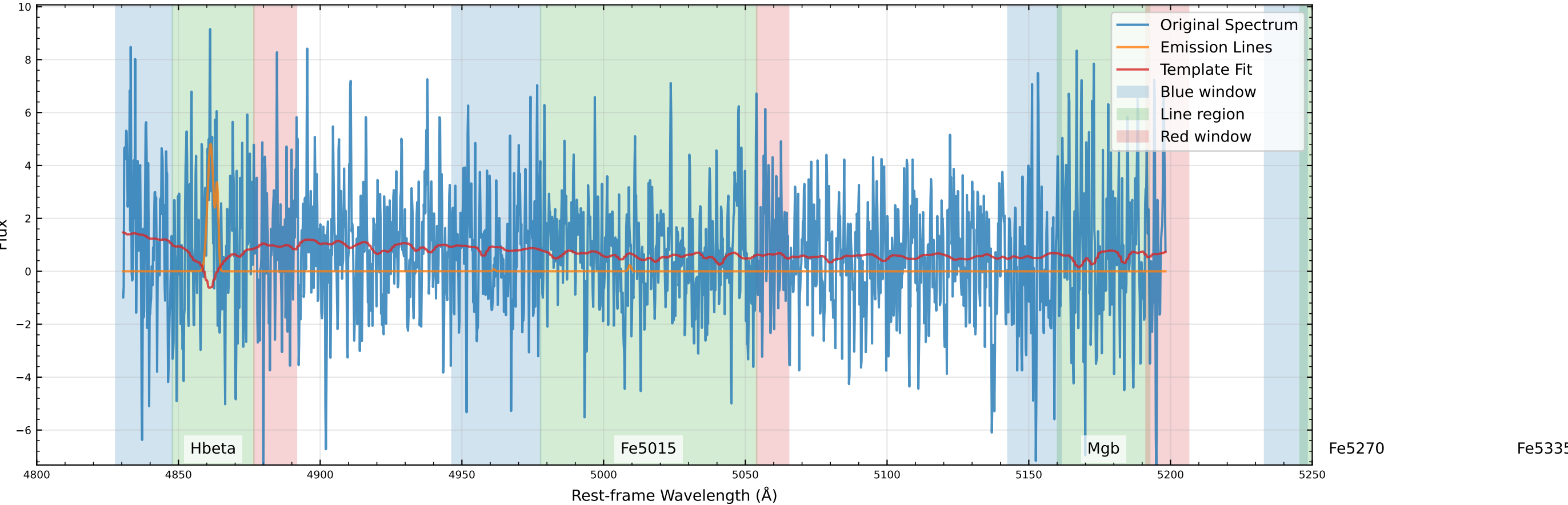
Original Data Comparison (v_star=149.3 km/s, v_gas=-27.1 km/s)
