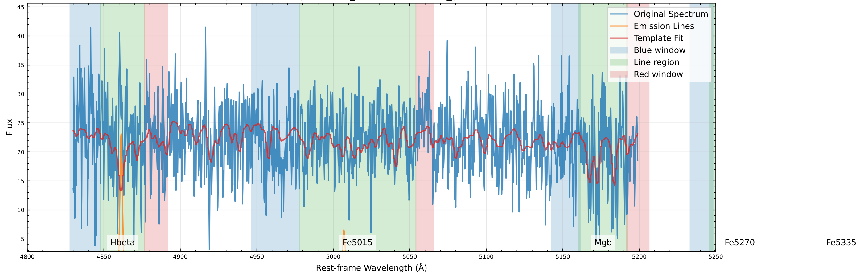
Original Data Comparison (v_star=-24.4 km/s, v_gas=-35.6 km/s)
